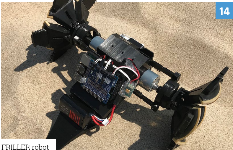
FRILLER robot
